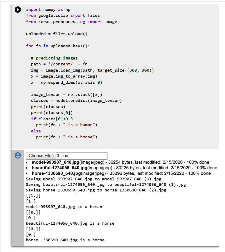
Figure 3-10. Executing the model
