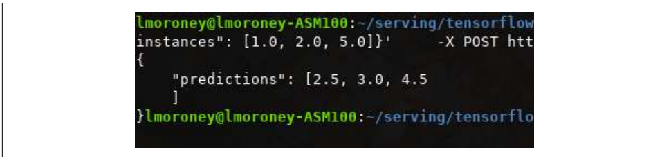
Figure 19-6. Results of running TensorFlow Serving
