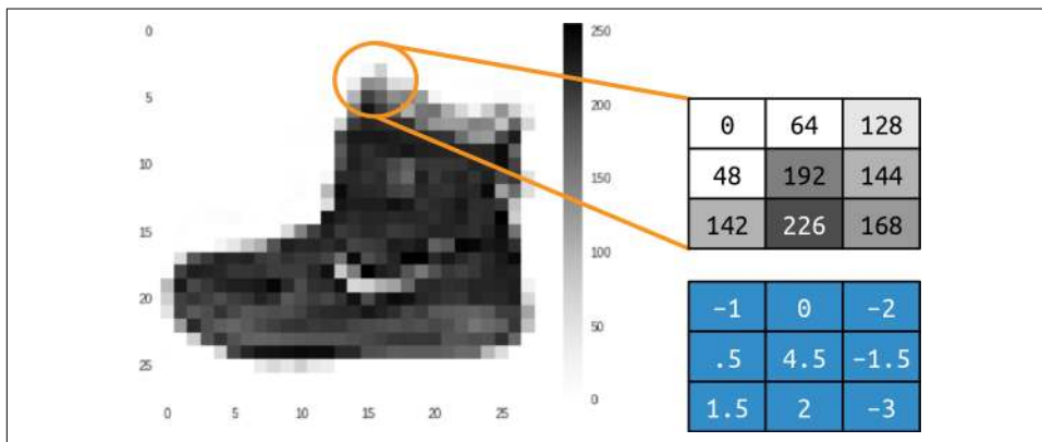
Figure 3-1. Ankle boot with convolution
